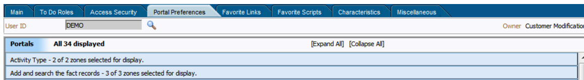
Figure 4–4 Portal Preferences
